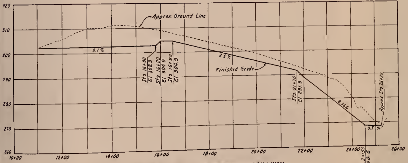
PROFILE ON \mathcal{C} OF EMERGENCY SPILLWAY
